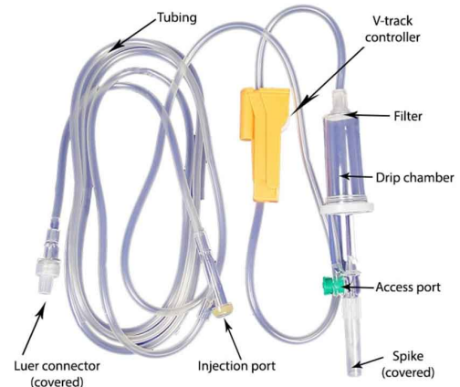
Components of IV Giving Set
